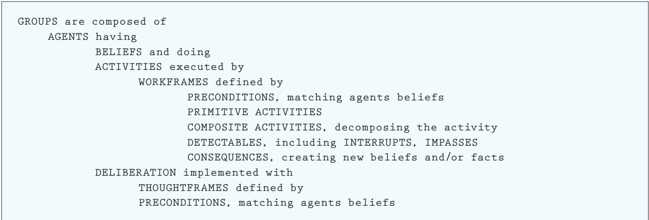
Figure 2. A simple taxonomy of some Brahms language concepts. These concepts form the basic building blocks in any Brahms project.
