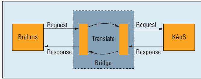
Figure 5. Schematic overview of the KAOs-Brahms bridge. A bidirectional translation is provided between KAOs concepts and Brahms concepts.
