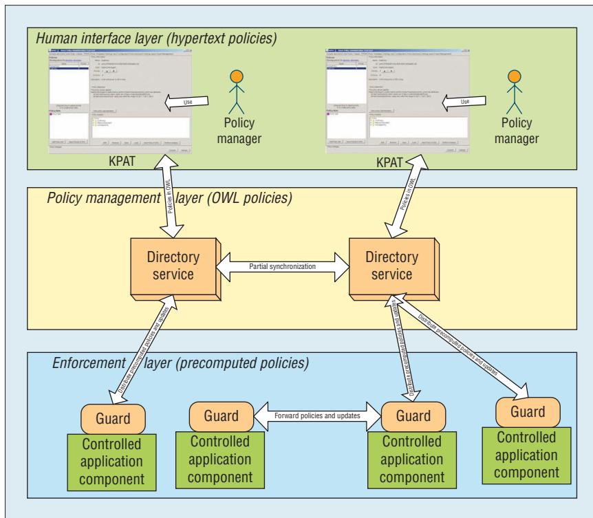
Figure 4. KAoS architecture. The human-interface, policy-management, and policy-monitoring and enforcement layers provide three different policy representations.
