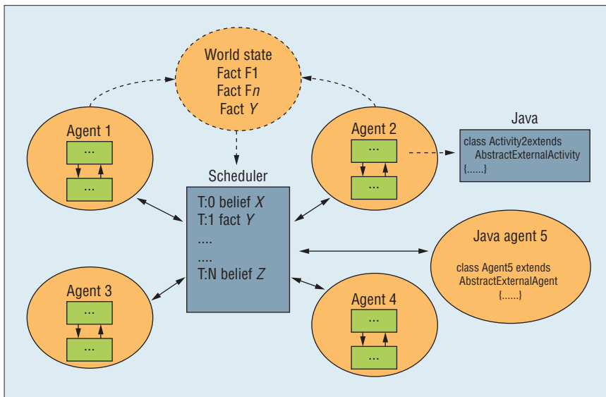
Figure 3. Brahms agent architecture. A Brahms simulation may run Brahms and Java agents.
