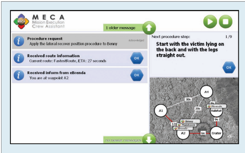
Figure 8. Human-in-the-loop interface. Messages are on the left, and procedure steps and a map with the actors are on the right.
